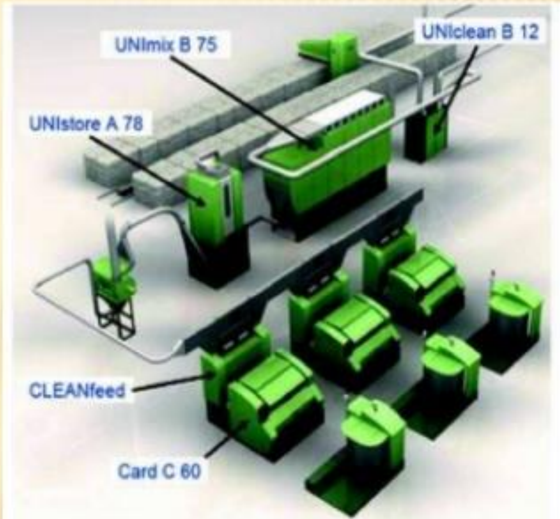
CLEAN-line consists of UNIfloc, UNIclean, UNImix, UNIstore and CLEANfeed
