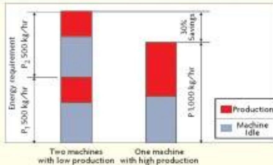
Figure 2: Energy savings with increased production
