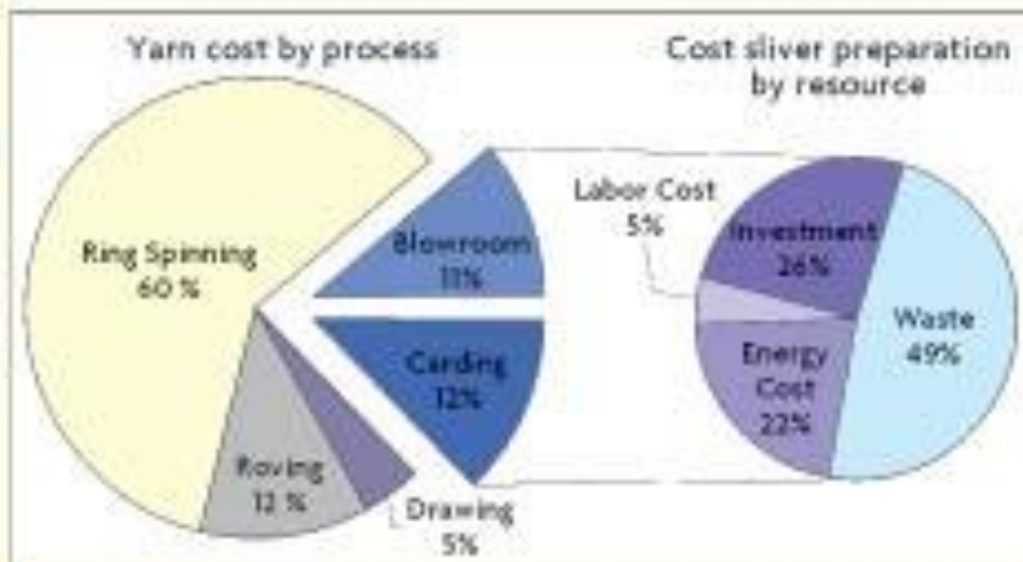
Figure 1: Manufacturing costs for Ne 30/1 yarn carded and sliver
