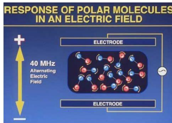
Figure 1. Operating principle of a radio frequency dryer.
